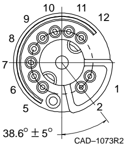
Figure 7 - Pin Connections and Rear View of Base EIA No. B10-301-BD
