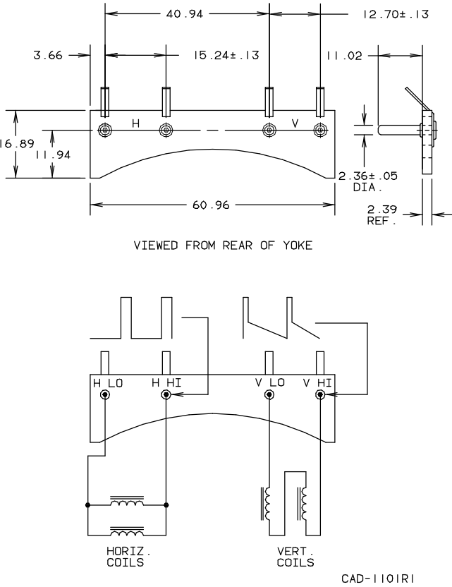
Figure 1 - Yoke Terminal Board and Connection Diagram, Top Board
