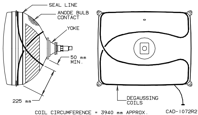
Figure 10 - Relative Placement of Typical Twisted Loop Degaussing Coils
