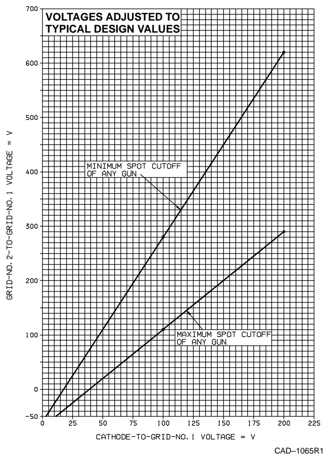
Figure 3 - Cutoff Design Chart
