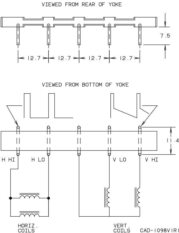
Figure 2 - Yoke Terminal Board and Connection Diagram, Bottom Board
