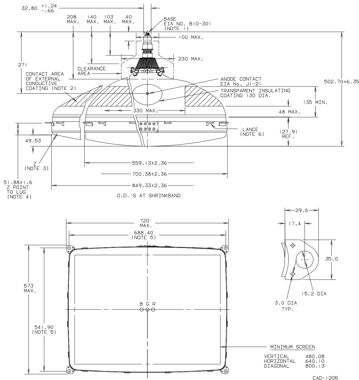
Figure 8 – Dimensional Outline (Dimensions in mm unless otherwise noted)
